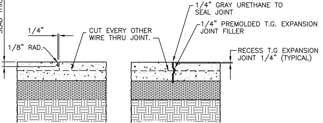
CONTROL JOINT (SPACED EVERY 5' TO 7')
