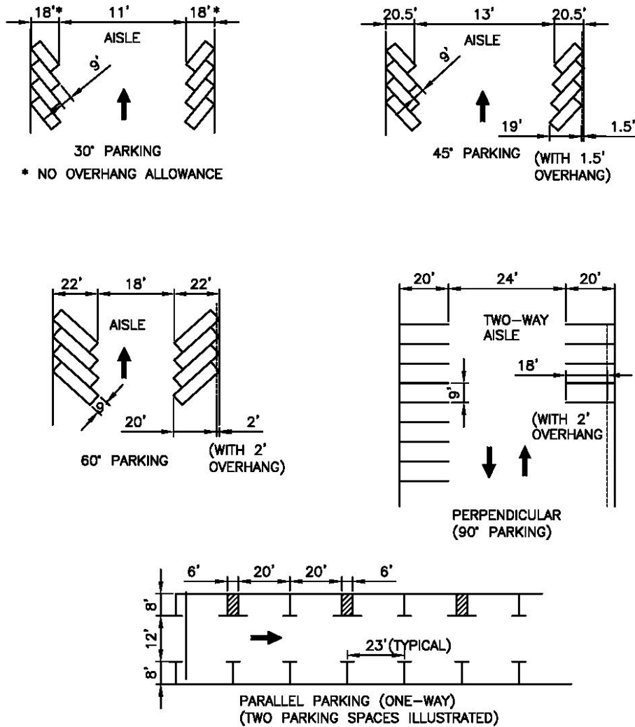
PARKING AREA DIMENSIONS (FOR STANDARD-SIZE VEHICLES)
